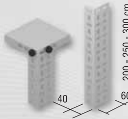
Çelik Raf Profil (40x60) Steel Shelf Profile (40x60)
